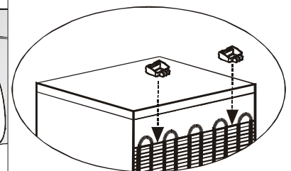
The scheme of installation of rear stoppers
